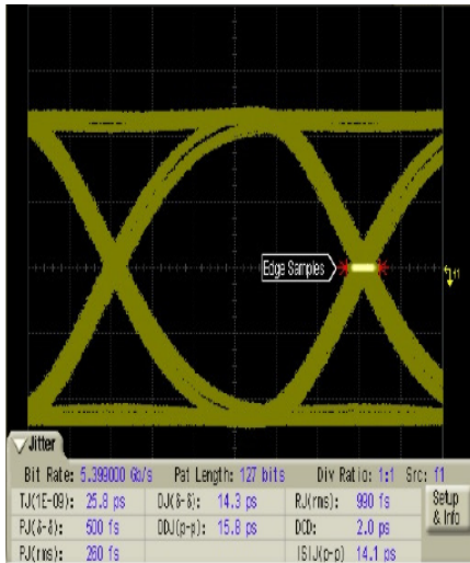
Figure 28. Eye Diagram (EQ = 6 dB)
