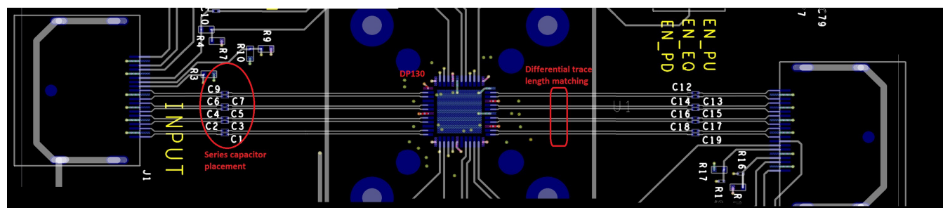
Figure 38. Layout Example
