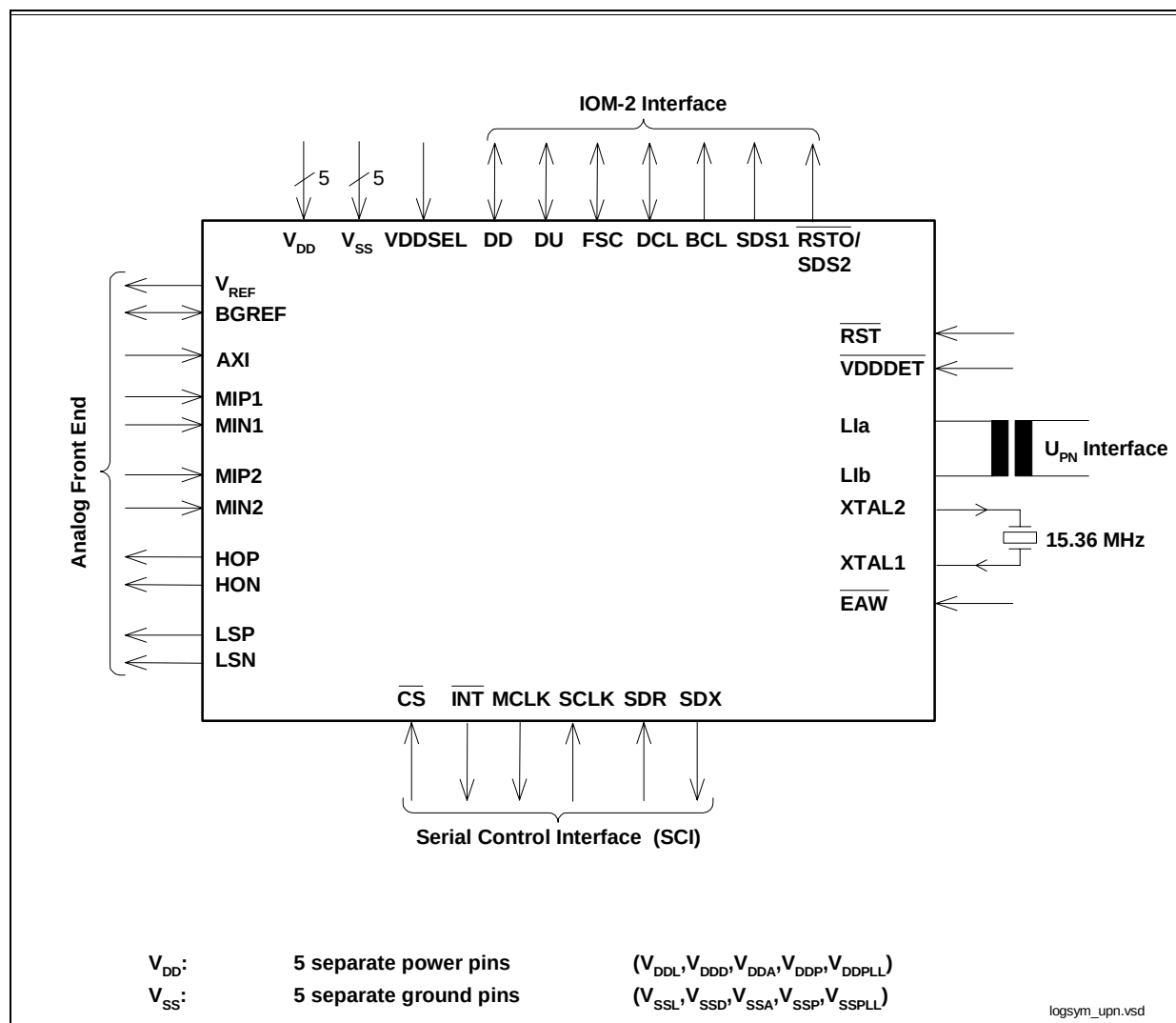
Figure 2 Logic Symbol of the SCOUT in P-MQFP-44
