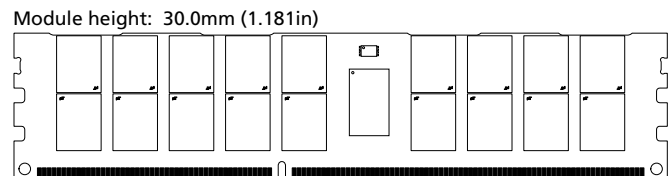
Figure 1: 240-Pin RDIMM (MO-269 R/C J)
