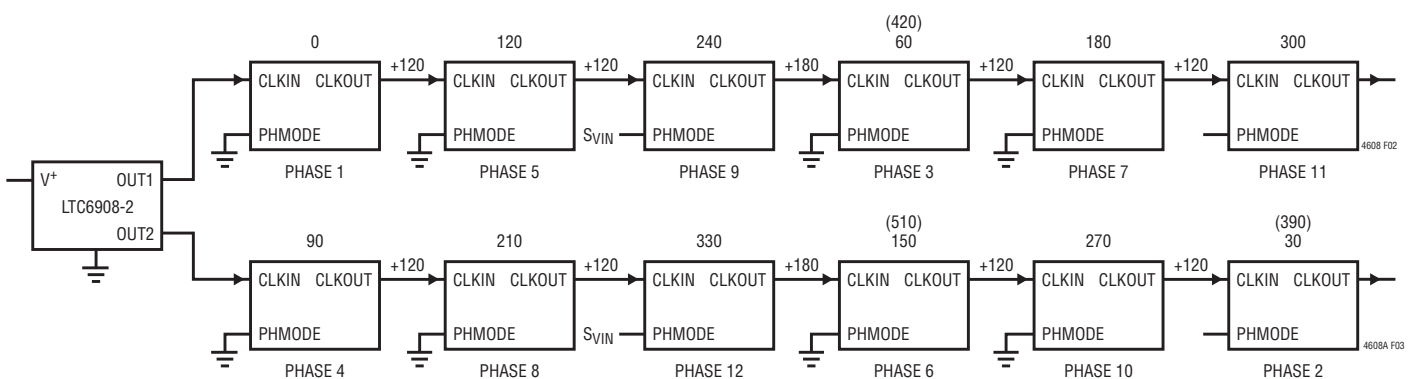
Figure 3. 12-Phase Operation
