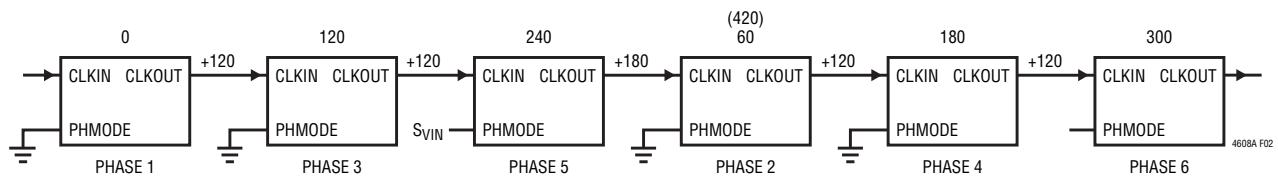
Figure 2. 6-Phase Operation
