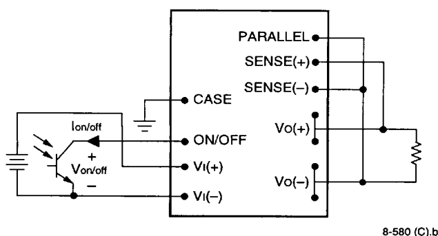
Figure 11. Remote On/Off Implementation
