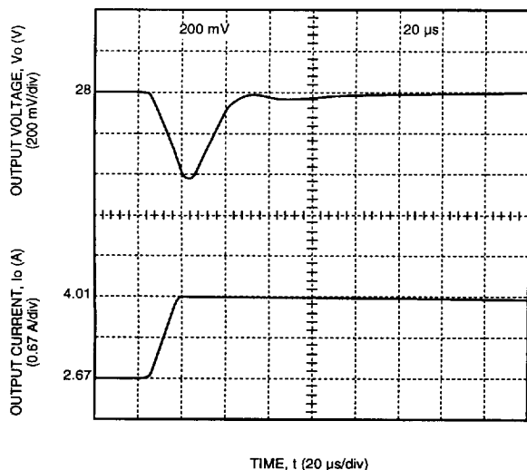
Figure 6. Typical FE150R Transient Response to Step Increase in Load from 50% to 75% of Full Load at Room Temperature and 48 V Input (Waveform Averaged to Eliminate Ripple Component.)
