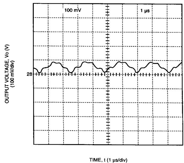
Figure 4. Typical FE150R Output Ripple Voltage at Room Temperature, 48 V Input, and 5.4 A Output
