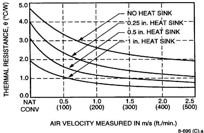
Figure 19. Heat Sink Resistance Curves; Fins Oriented Along Width
