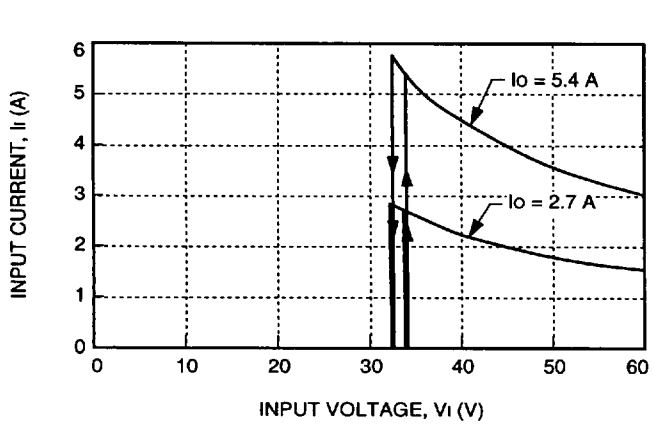
Figure 1. Typical FE150R Input Characteristics at Room Temperature
