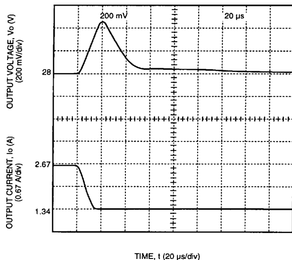
Figure 5. Typical FE150R Transient Response to Step Decrease in Load from 50% to 25% of Full Load at Room Temperature and 48 V Input (Waveform Averaged to Eliminate Ripple Component.)
