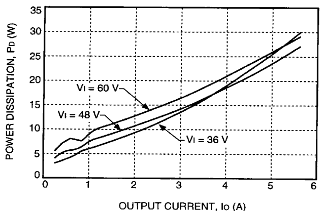
Figure 21. FE150R Power Dissipation as Heat vs. Output Current
