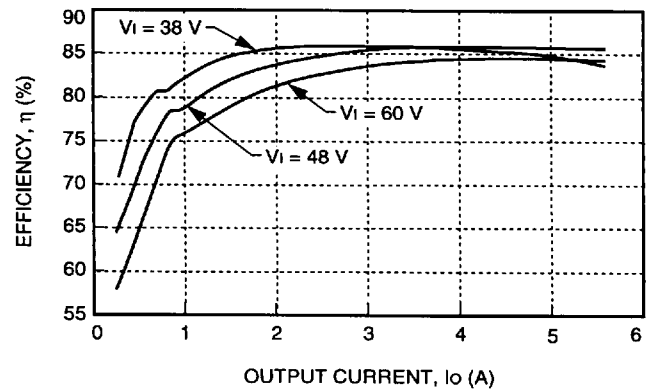
Figure 3. Typical FE150R Efficiency vs. Output Current at Room Temperature
