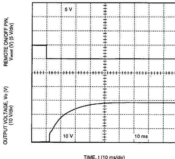
Figure 7. Typical FE150R Start-Up Transient at Room Temperature, 48 V Input, and 5.4 A Output
