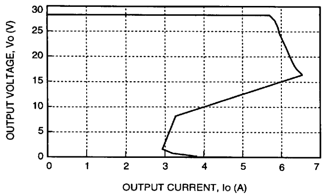
Figure 2. Typical FE150R Output Characteristics at Room Temperature and 48 V Input
