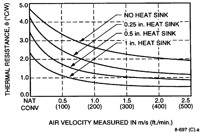
Figure 20. Heat Sink Resistance Curves; Fins Oriented Along Length
