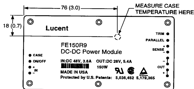
Figure 17. Case Temperature Measurement Location
