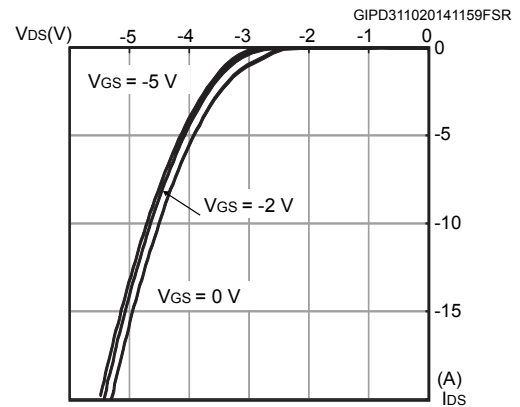
Figure 6. Body diode characteristics @ T_J = -50^\circ C
