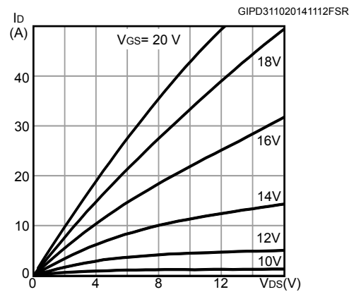
Figure 3. Output characteristics @ T_J = 25^\circ C
