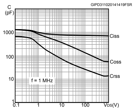
Figure 14. Capacitances variation
