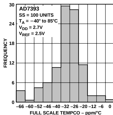
Figure 9. AD7393 Full-Scale Output Tempco Histogram
