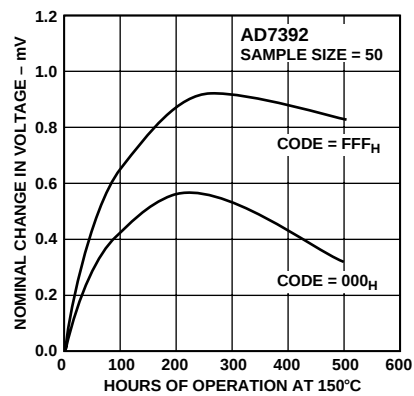
Figure 22. Long-Term Drift Accelerated by Burn-in
