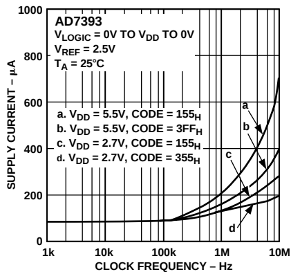
Figure 14. Supply Current vs. Clock Frequency
