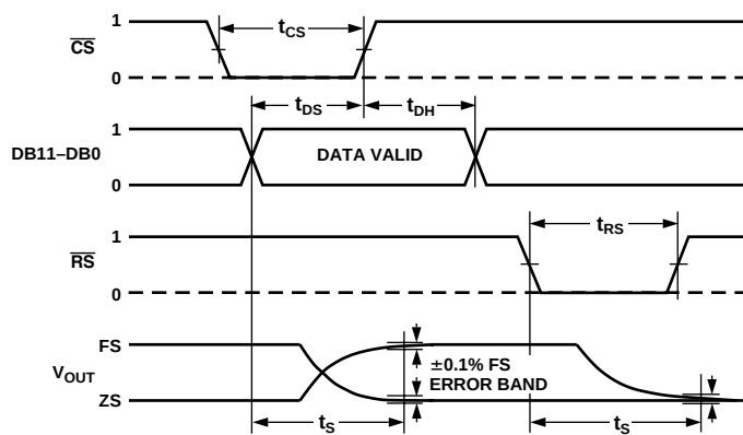
Figure 3. Timing Diagram
