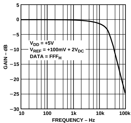
Figure 20. Reference Multiplying Bandwidth
