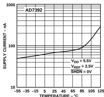
Figure 24. Shutdown Current vs. Temperature
