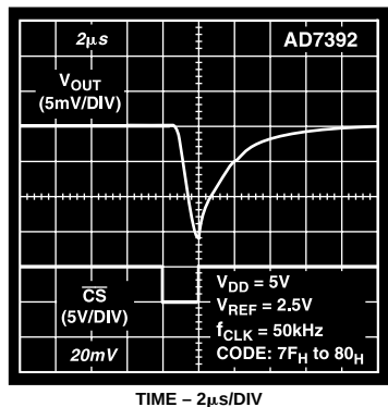
Figure 17. Midscale Transition Performance
