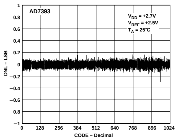
Figure 2. AD7393 Differential Nonlinearity Error vs. Code
