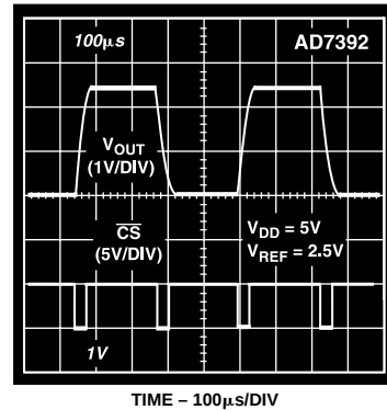
Figure 19. Large Signal Settling Time
