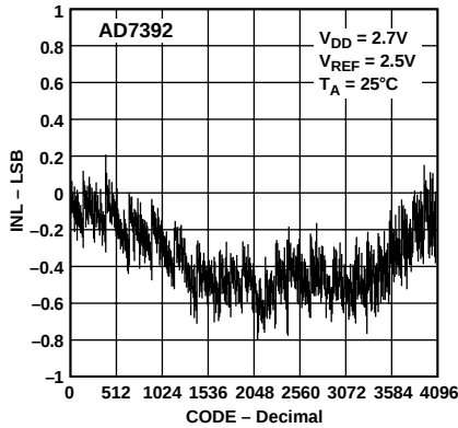
Figure 5. AD7392 Integral Nonlinearity Error vs. Code
