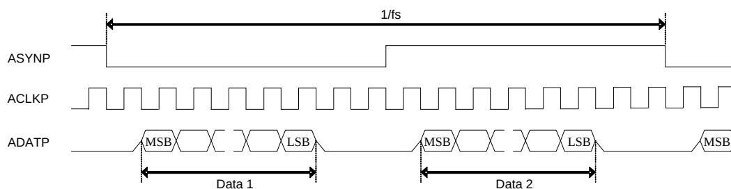
FIGURE 28. RM_SYNC=0, PB_MASTER=0, ADATPDLY=0
