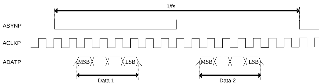
FIGURE 34. RM_SYNC=0,PB_MASTER=0,ADATPDLY=0
