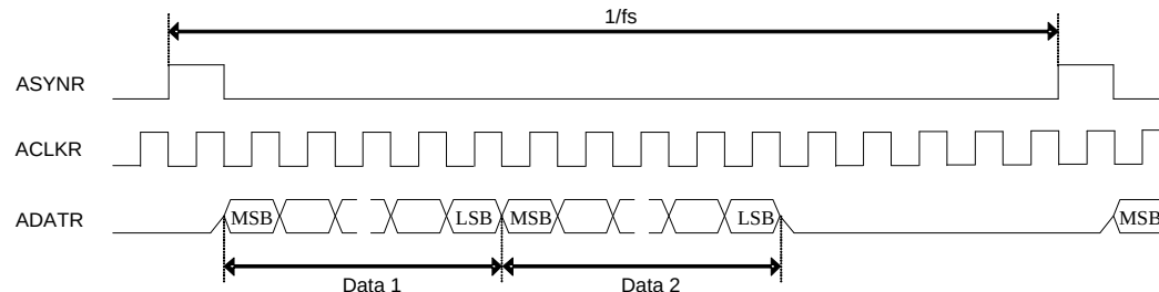
FIGURE 25. ACLKMASTER=0, RM_SYNC=1
