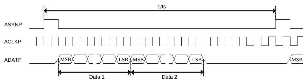
FIGURE 29. RM_SYNC=1, PB_MASTER=0, ADATPDLY=0
