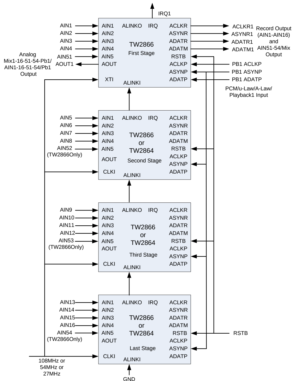
FIGURE 20. RECOMMENDED CLOCK MASTER CASCADE MODE SYSTEM
