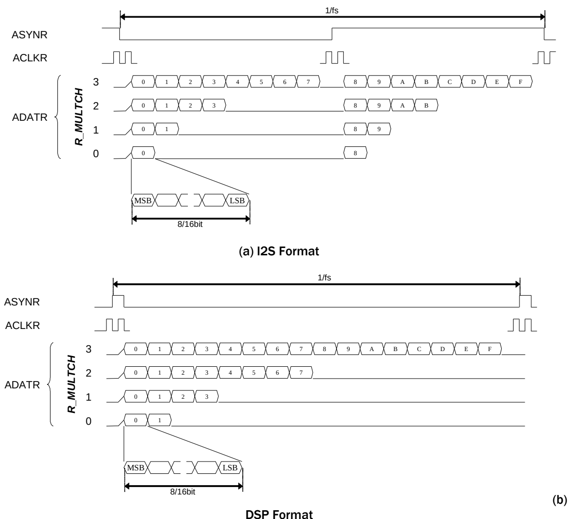
FIGURE 23. TIMING CHART OF MULTI-CHANNEL AUDIO RECORD
