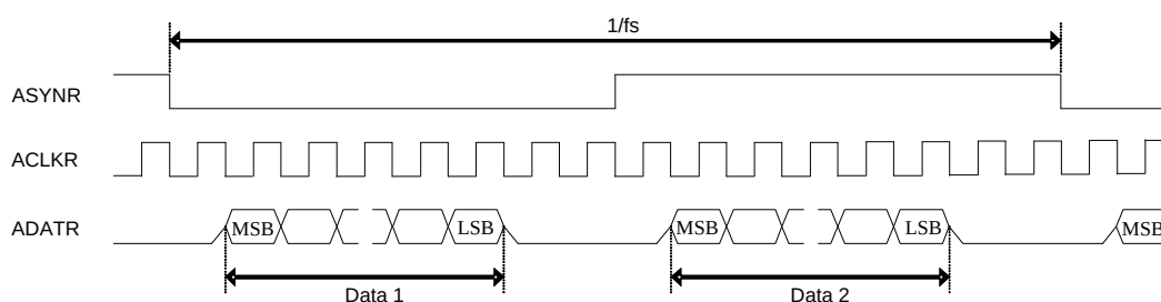
FIGURE 24. ACLKMASTER=0, RM_SYNC=0
