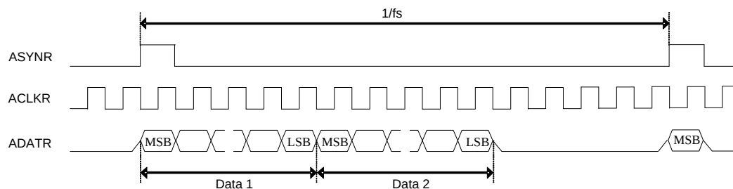
FIGURE 31. RM_SYNC=1,PB_MASTER=0,ADATPDLY=1
