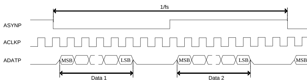
FIGURE 32. RM_SYNC=0,PB_MASTER=0,ADATPDLY=1
