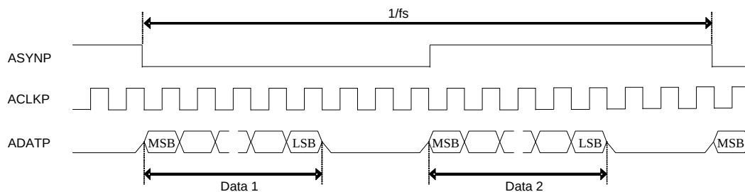
FIGURE 30. RM_SYNC=0, PB_MASTER=0, ADATPDLY=1
