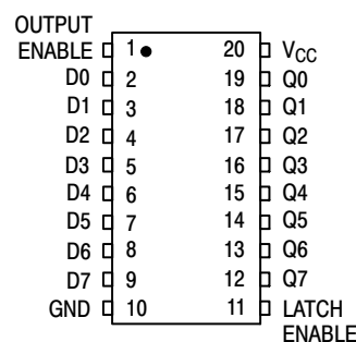
SOIC-20 DW SUFFIX CASE 751D
