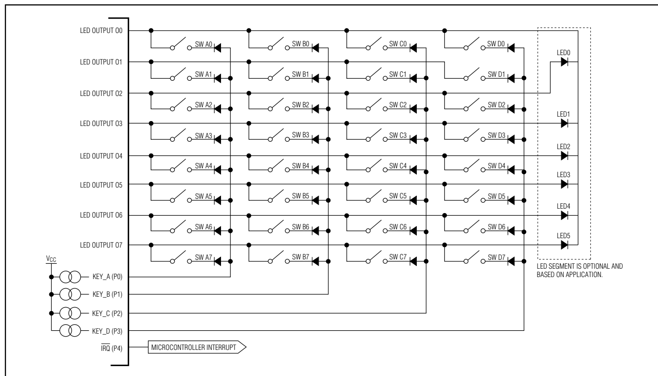
Figure 11. Key-Scanning Configuration
