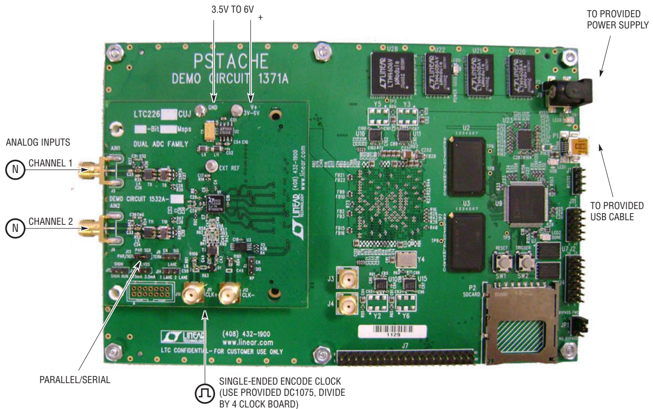
Figure 1. DC1532A Setup
