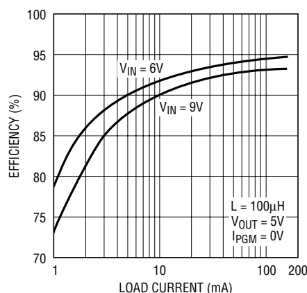
LTC1174-5 Efficiency
