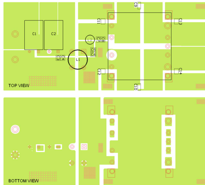
Recommended Layout With Input Filter
