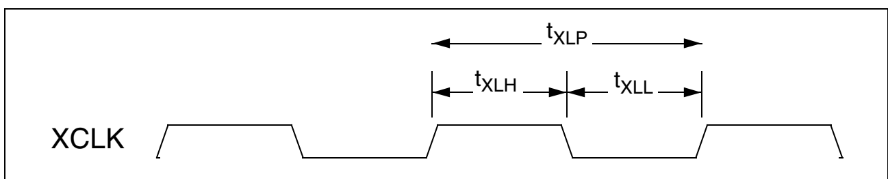
Figure 90 XCLK Timing
