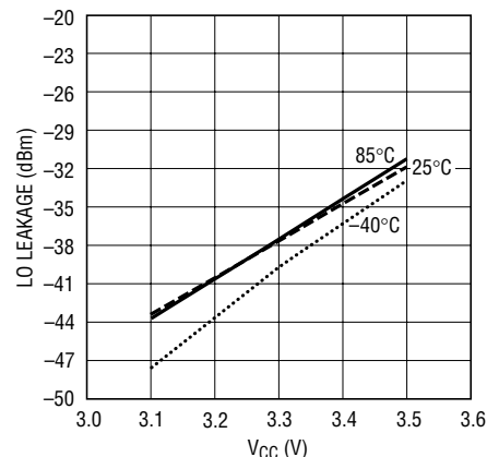
LO Leakage vs Supply Voltage
