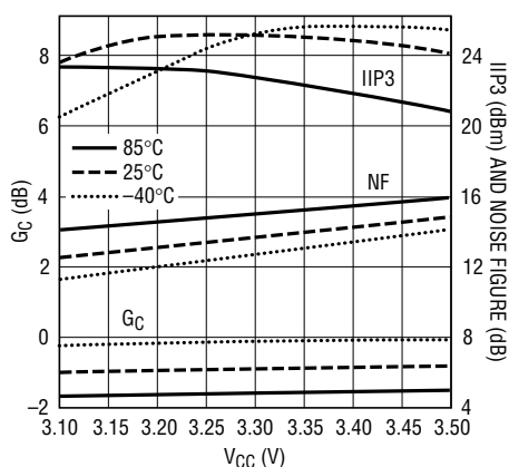
Conversion Gain, IIP3 and Noise Figure vs Supply Voltage
