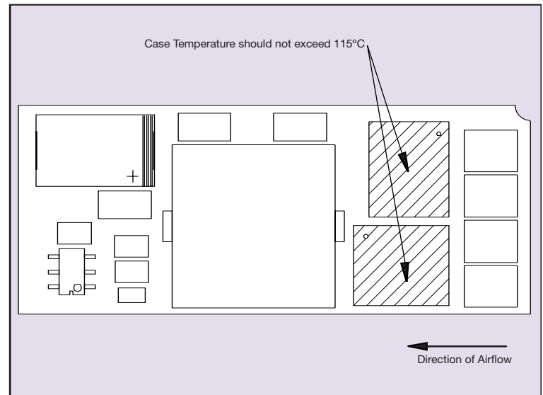
Figure 26: Thermal Reference Points
