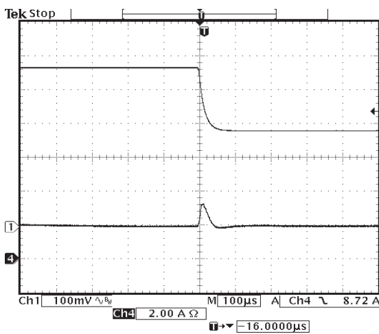
Figure 13: Typical Transient Response 75% - 50% Step Load Change (Channel 1: V_o , Channel 4: I_o )
