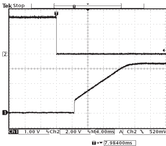
Figure 15: Control On/Off Characteristic (Channel 1: Vo, Channel 2: Remote ON/OFF)
