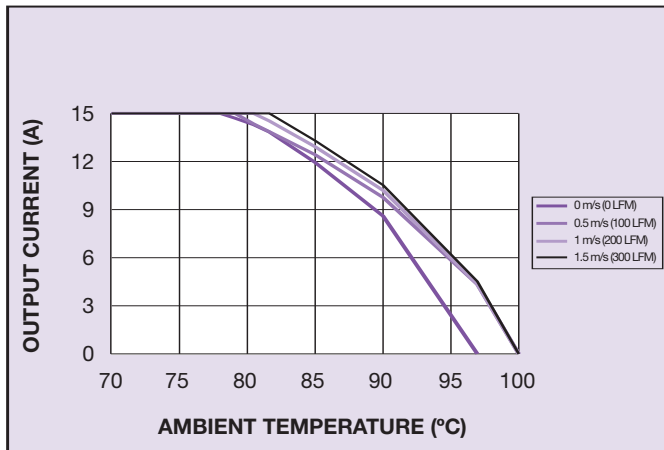
Figure 1: Derating Curve with V_{in} = 5V and No Trim
