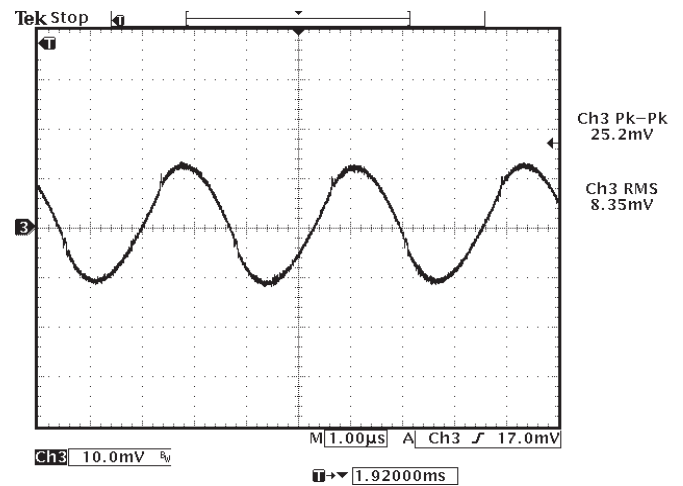
Figure 8: Typical Ripple and Noise* (Channel 3: Vo)
