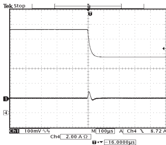
Figure 5: Typical Transient Response 75% - 50% Step Load Change (Channel 1: V_o , Channel 4: I_o )
