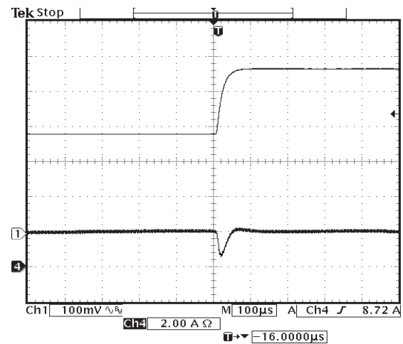
Figure 12: Typical Transient Response 50% - 75% Step Load Change (Channel 1: V_o , Channel 4: I_o )
