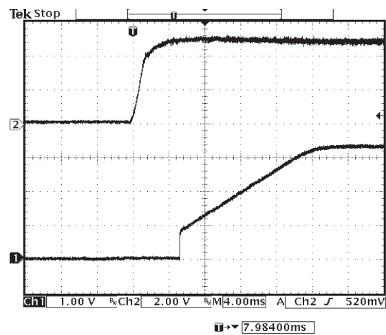
Figure 14: Typical Power-up Characteristic (Channel 1: V_o , Channel 2: V_{in} )
