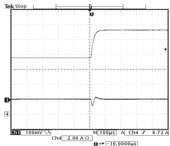
Figure 4: Typical Transient Response 50% - 75% Step Load Change (Channel 1: V_o , Channel 4: I_o )
