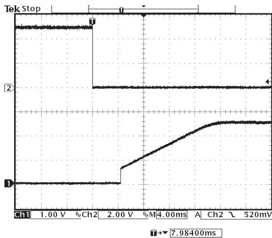
Figure 7: Control On/Off Characteristic (Channel 1: Vo, Channel 2: Remote ON/OFF)
