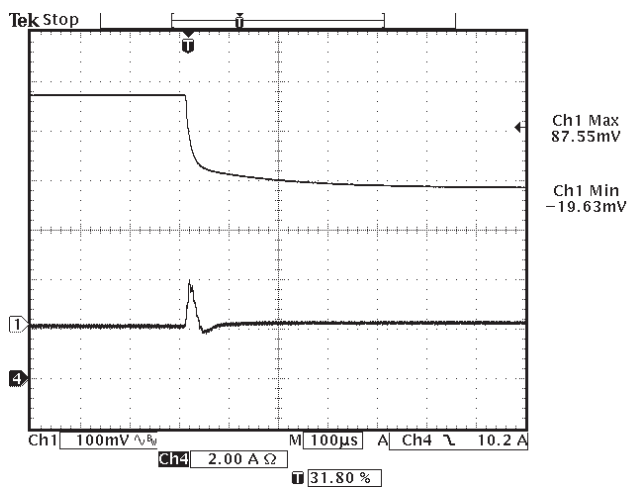
Figure 21: Typical Transient Response 75% - 50% Step Load Change (Channel 1: V_o , Channel 4: I_o )
