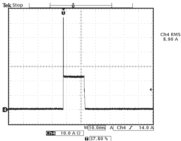
Figure 19: Short Circuit Characteristic (Channel 4: I_o )
