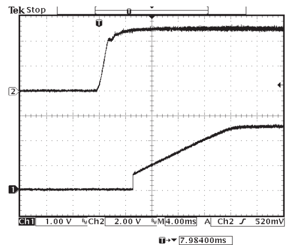
Figure 6: Typical Power-up Characteristic (Channel 1: V_o , Channel 2: V_{in} )
