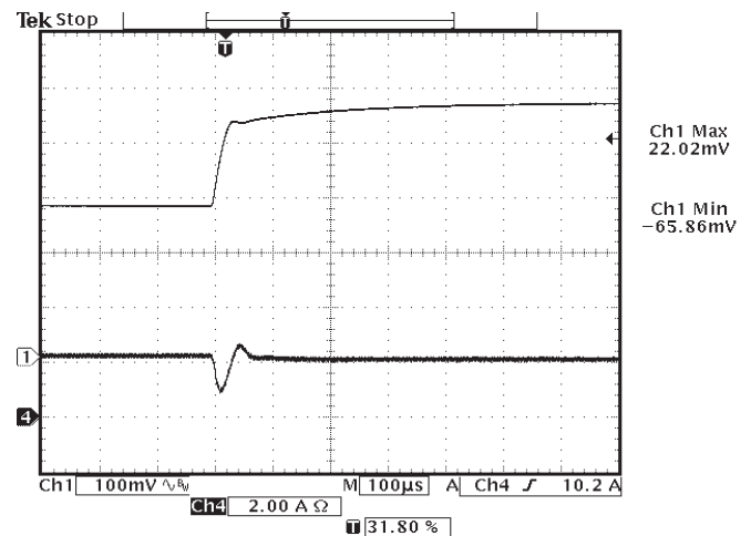
Figure 20: Typical Transient Response 50% - 75% Step Load Change (Channel 1: V_o , Channel 4: I_o )
