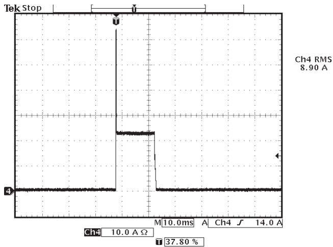
Figure 11: Short Circuit Characteristic (Channel 4: I_o )
