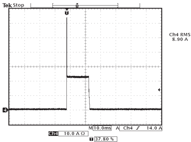
Figure 3: Short Circuit Characteristic (Channel 1: I_{s/c} )
