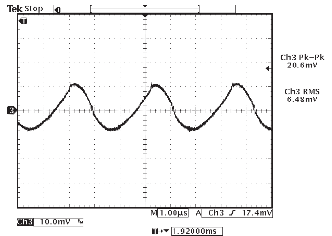
Figure 16: Typical Ripple and Noise* (Channel 3: Vo)
