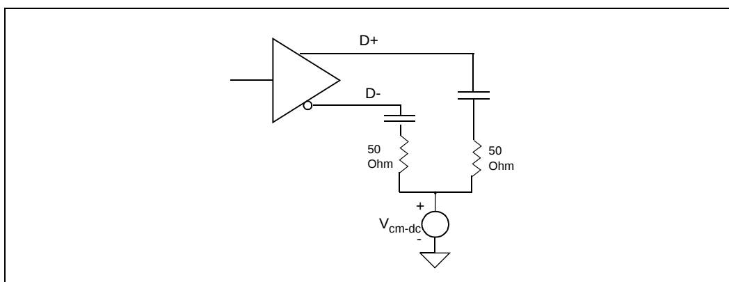
Figure 19. Transmitter Test Load (100 Ω differential load)
