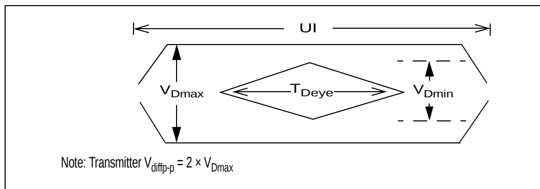
Figure 21. Receiver Eye Opening (Differential)
