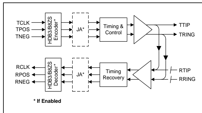
Figure 8. Analog Loopback
