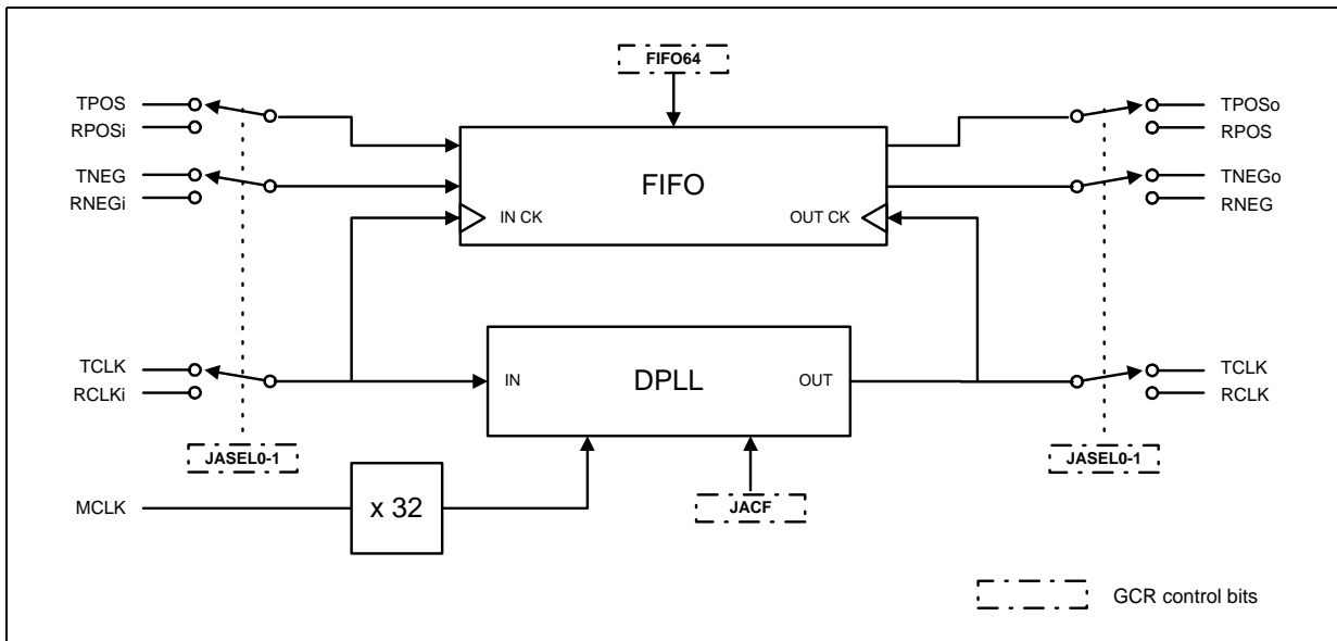
Figure 7. Jitter Attenuator Loop
