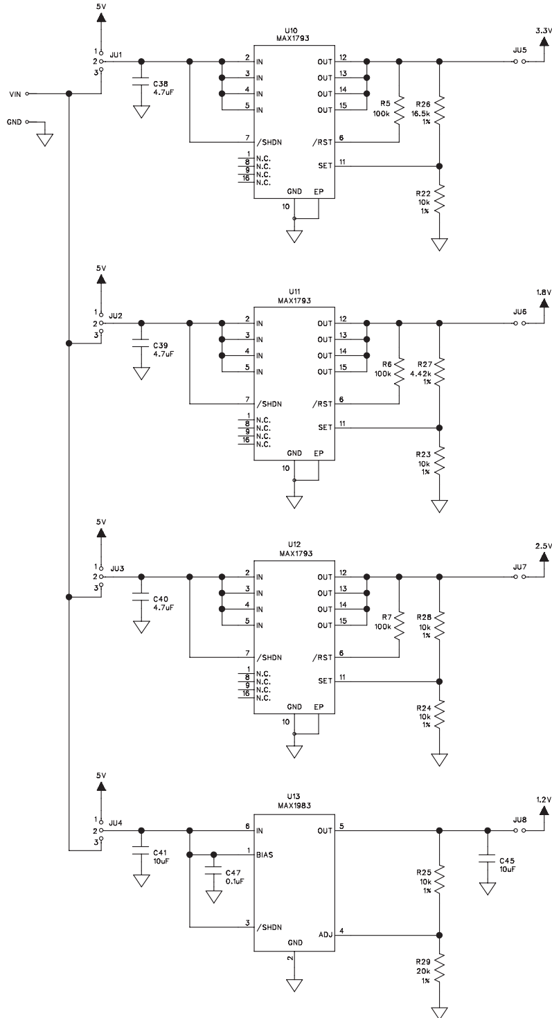
Figure 6k. MAX11666 EV Kit Schematic (Sheet 11 of 12)
