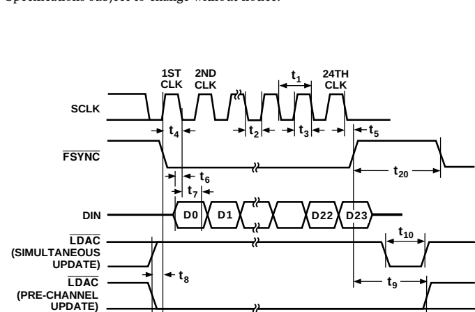
Figure 1. AD7834 Timing Diagram
