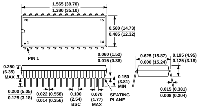
28-Leaded Plastic DIP (N-28)
