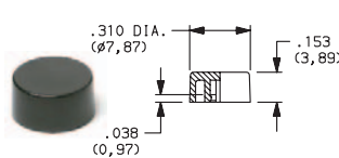
Cap Compatible with snap-fitting plungers EP11 & EP12 Models
