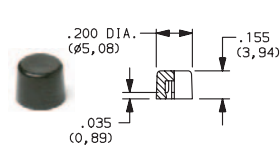
Cap Compatible with snap-fitting plungers EP11 & EP12 Models
