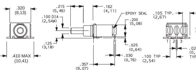
EP11 Models: omit terminal 2.
