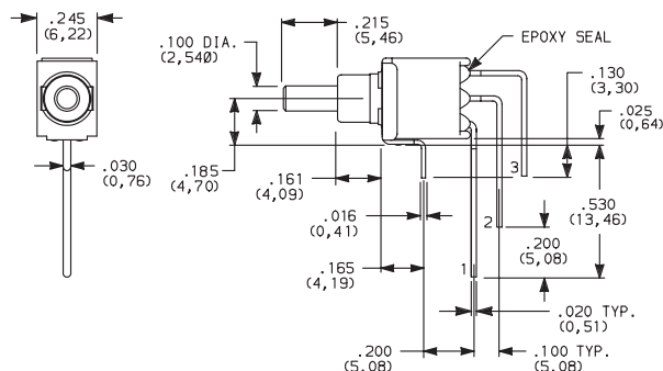
EP11 Models: omit terminal 2.
