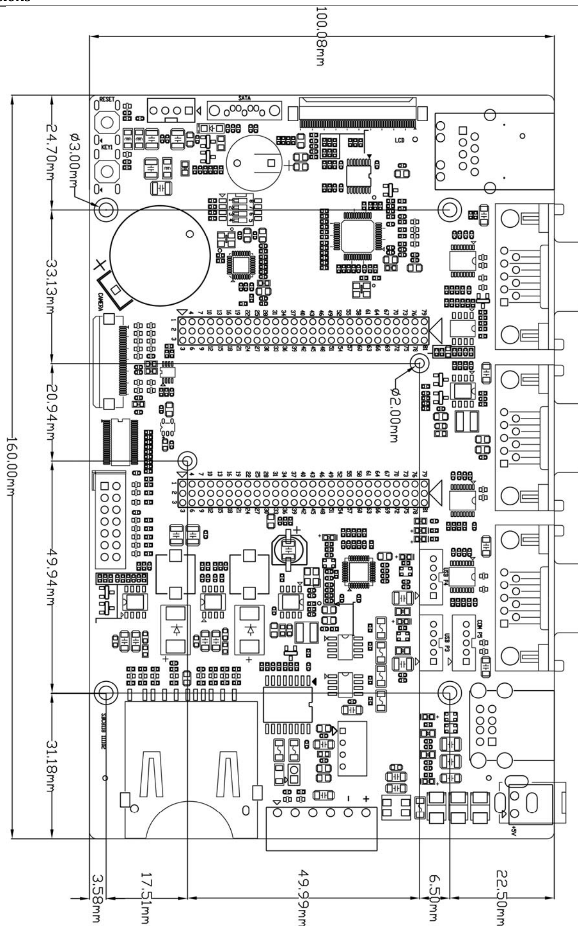
Dimension Chart of SBC8118 Single Board Computer
