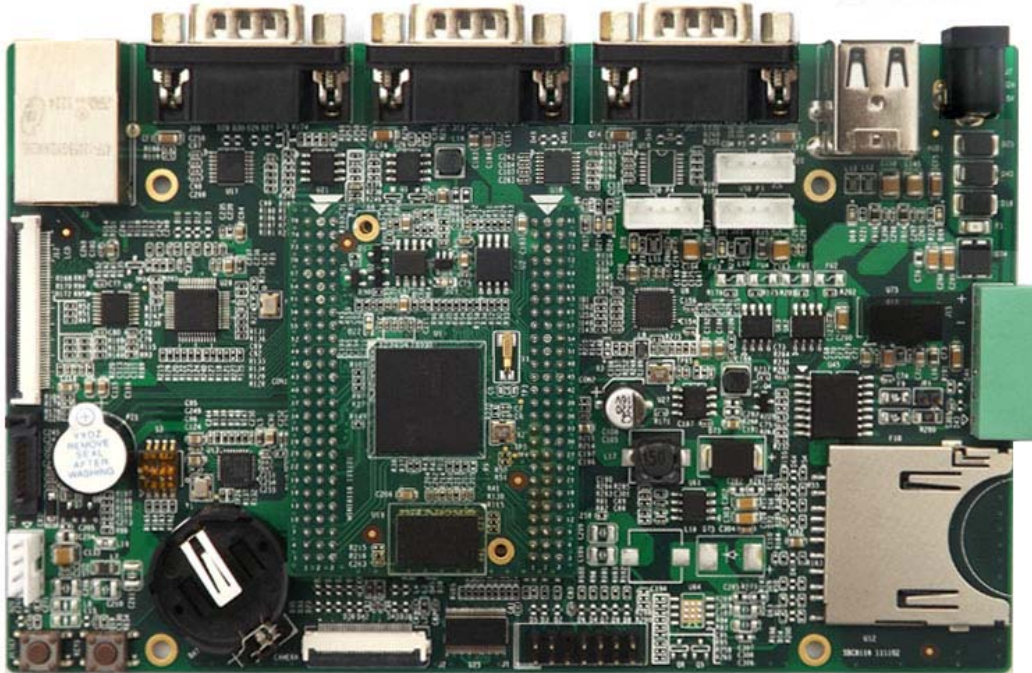
SBC8118 Single Board Computer
