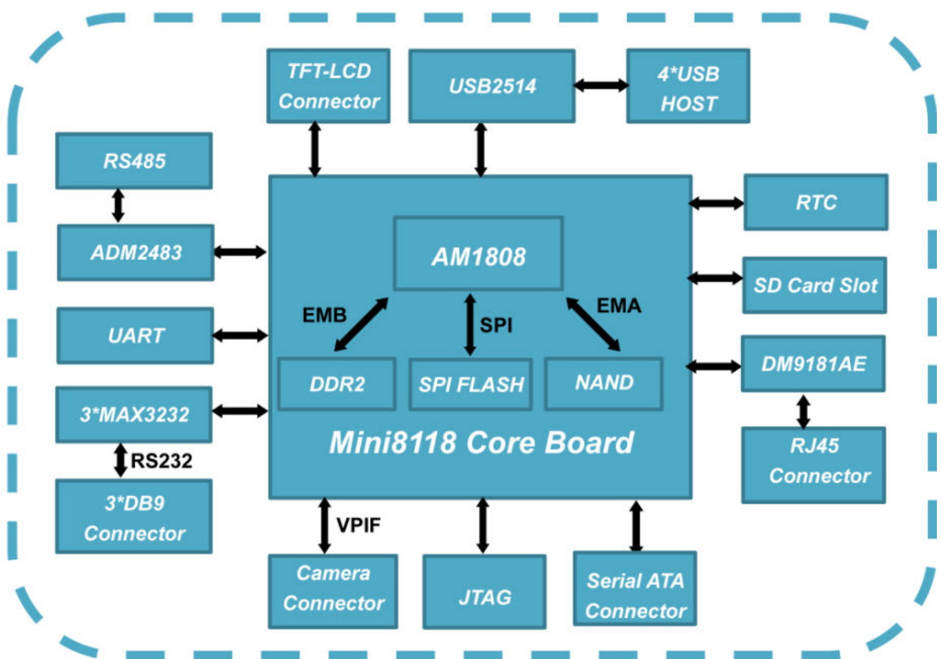
SBC8118 Function Block Diagram
