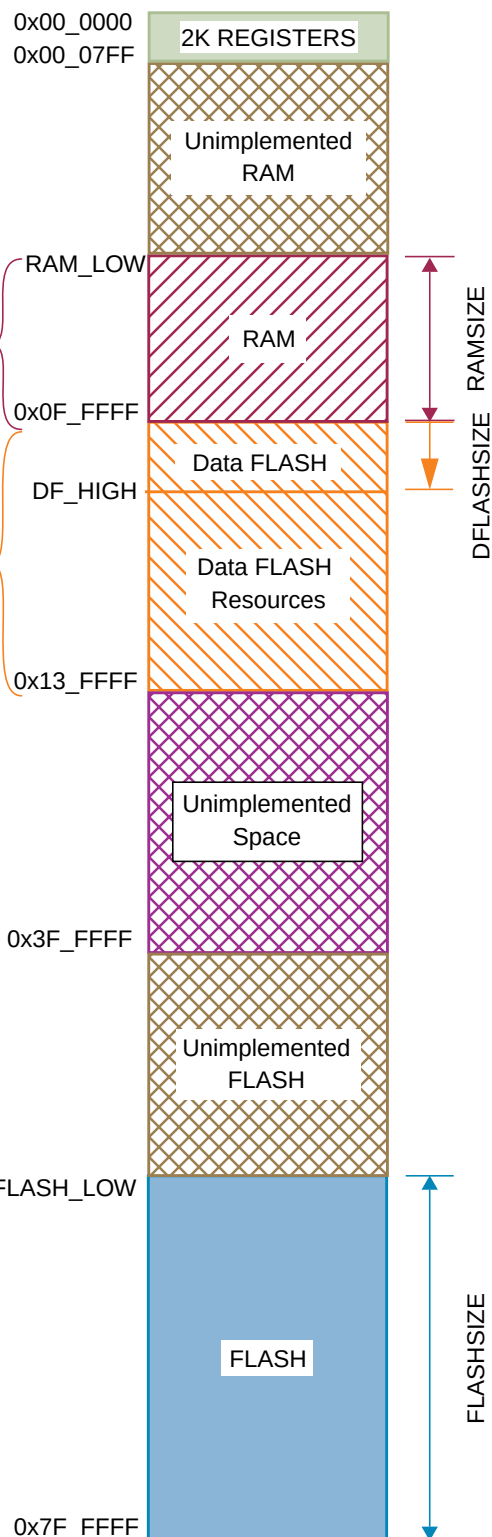
Figure 3-19. S12X CPU &amp; BDM Global Address Mapping
