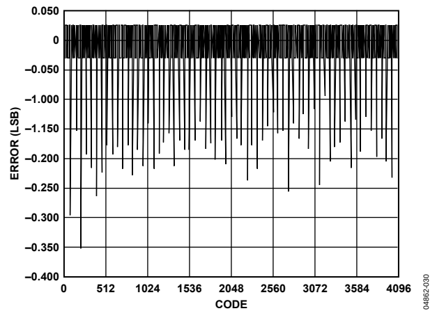
Figure 32. AD9735 DNL, 25°C, 30 mA FS
