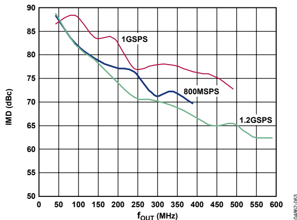
Figure 62. AD9734 IMD vs. f_{OUT} over f_{DAC} , 1.2 GSPS
