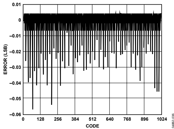
Figure 38. AD9734 DNL, 25°C, 30 mA FS
