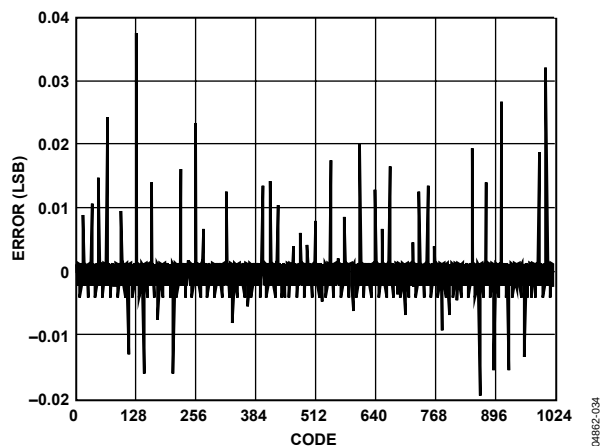
Figure 36. AD9734 DNL, 25°C, 10 mA FS
