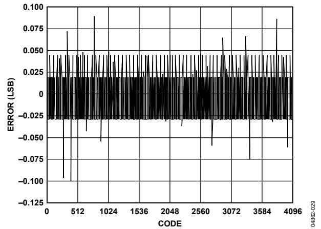
Figure 31. AD9735 DNL, 25°C, 20 mA FS
