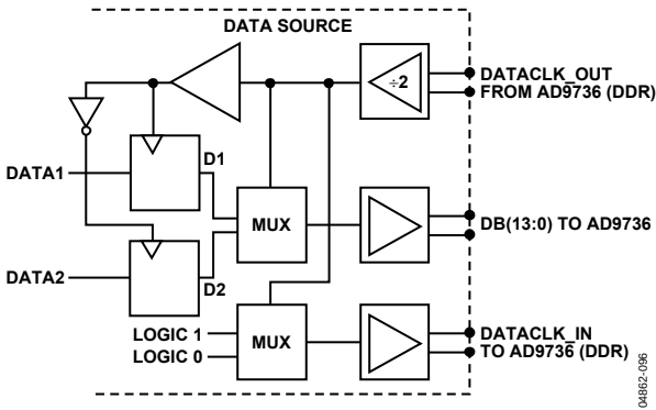
Figure 98. Recommended FPGA/ASIC Configuration for Driving AD9736 Digital Inputs, 2x Mode
