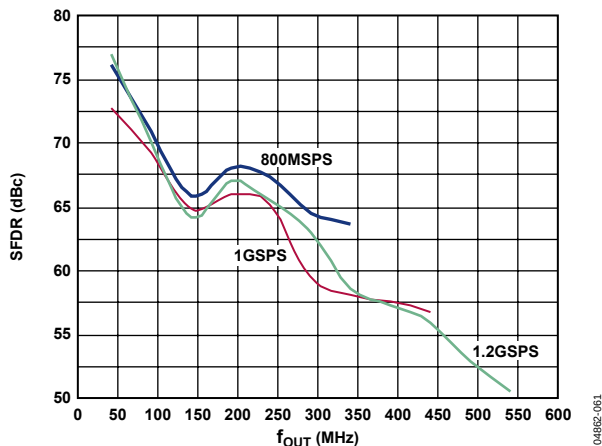
Figure 60. AD9734 SFDR vs. f_{OUT} over f_{DAC} , 1.2 GSPS
