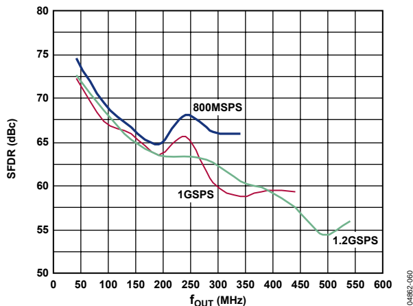
Figure 59. AD9735 SFDR vs. f_{OUT} over f_{DAC} , 1.2 GSPS
