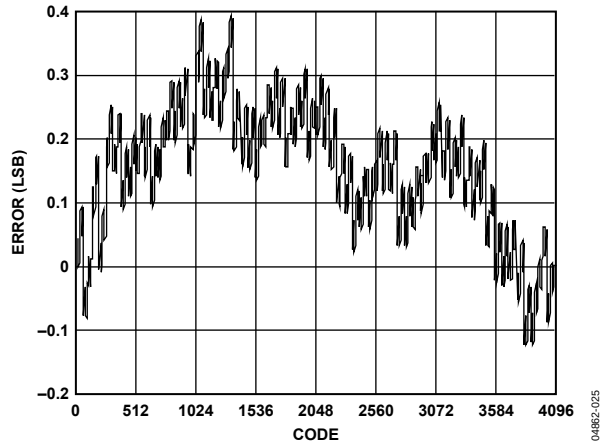
Figure 27. AD9735 INL, 25°C, 10 mA FS
