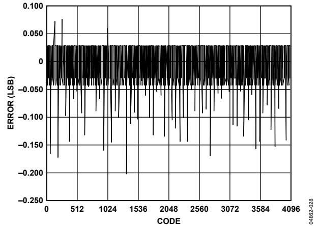
Figure 30. AD9735 DNL, 25°C, 10 mA FS
