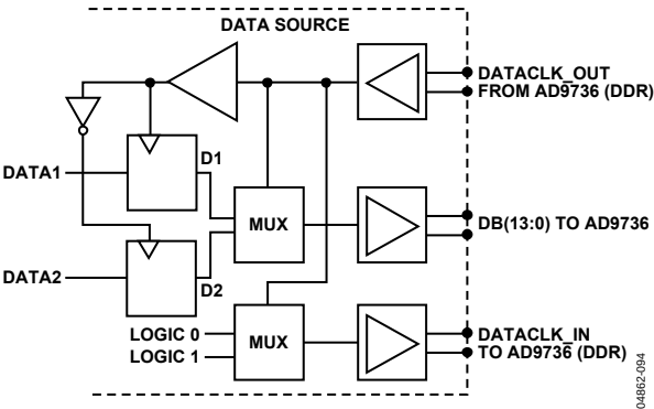
Figure 96. Recommended FPGA/ASIC Configuration for Driving AD9736 Digital Inputs, 1x Mode
