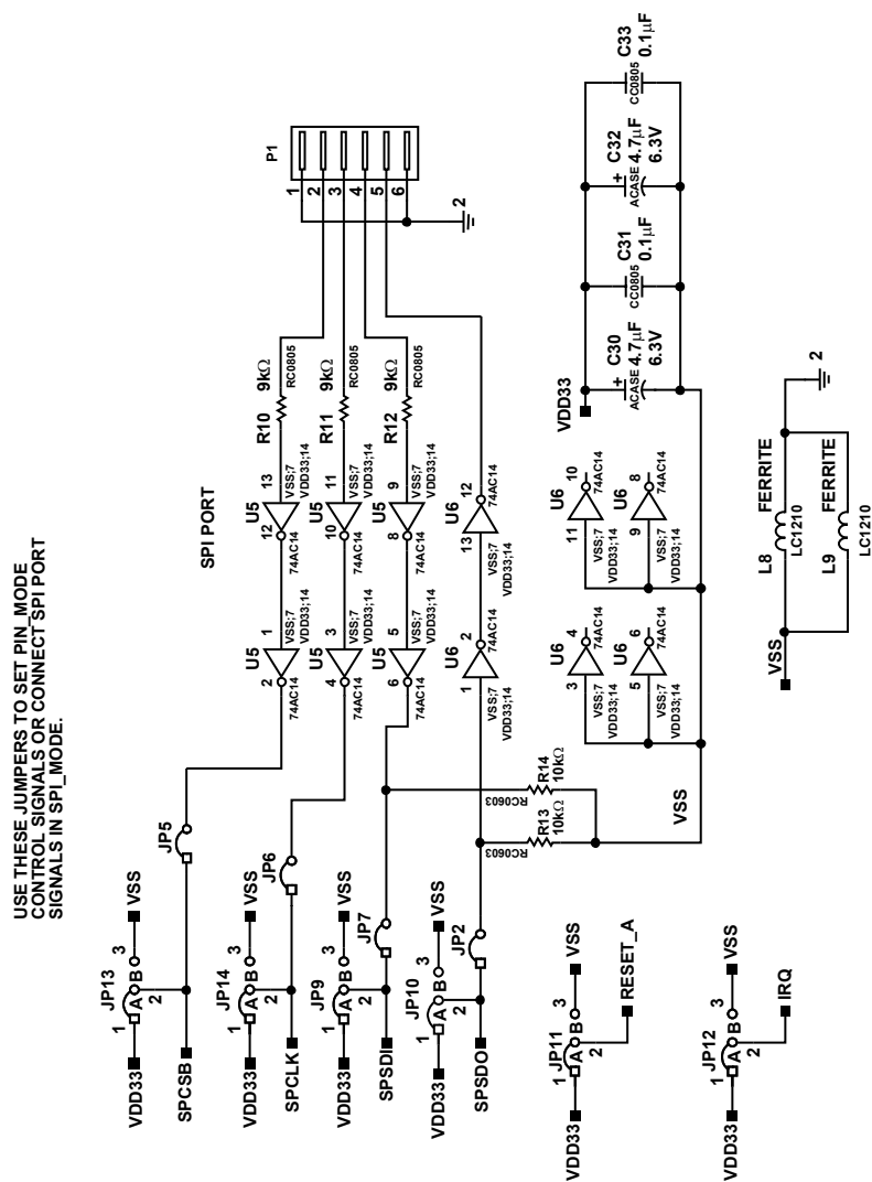
Figure 108. SPI Port Interface, AD973x Evaluation Board, Rev. F
