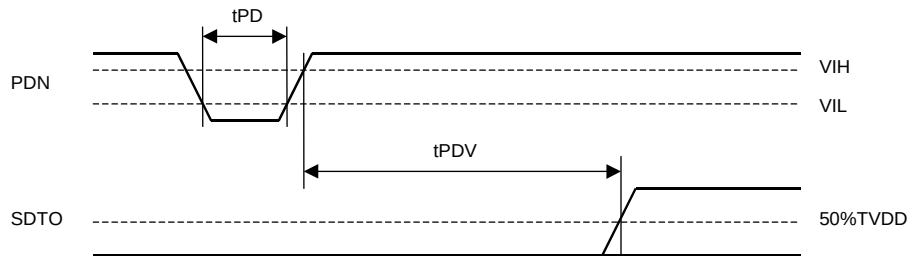
Power-down &amp; Reset Timing
