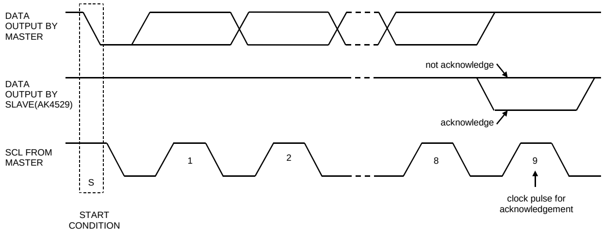
Figure 23. Acknowledge on the I²C-bus
