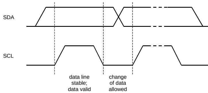
Figure 24. Bit transfer on the I²C-bus
