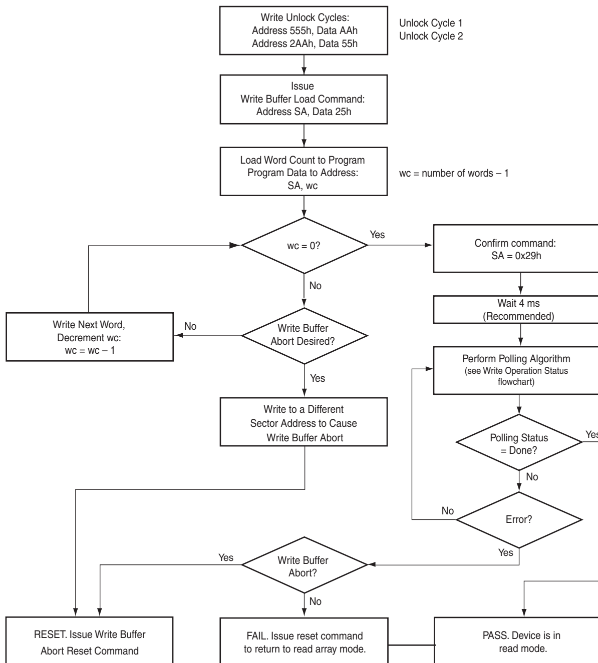
Figure 7.2 Write Buffer Programming Operation
