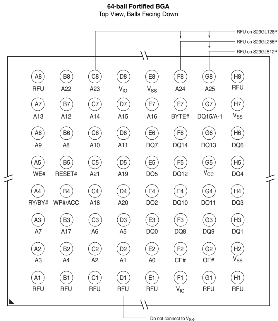
Figure 4.1 64-ball Fortified Ball Grid Array
