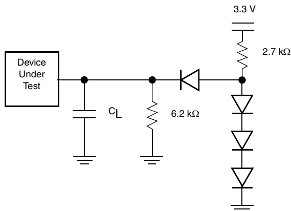
Figure 11.3 Test Setup
