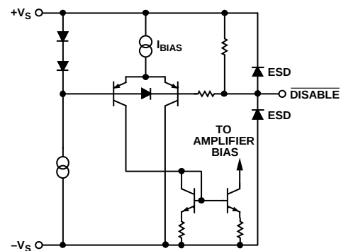
Figure 45. DISABLE Circuit
