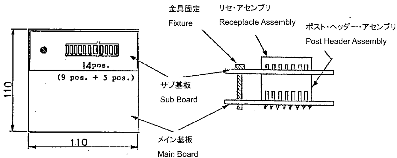
Fig.3 低周波振動の嵌合取付状態 Mated Condition for Low Frequency Vibration
