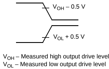
Figure 5. Test Point Levels for Driven-to-Three-State Time Measurements
