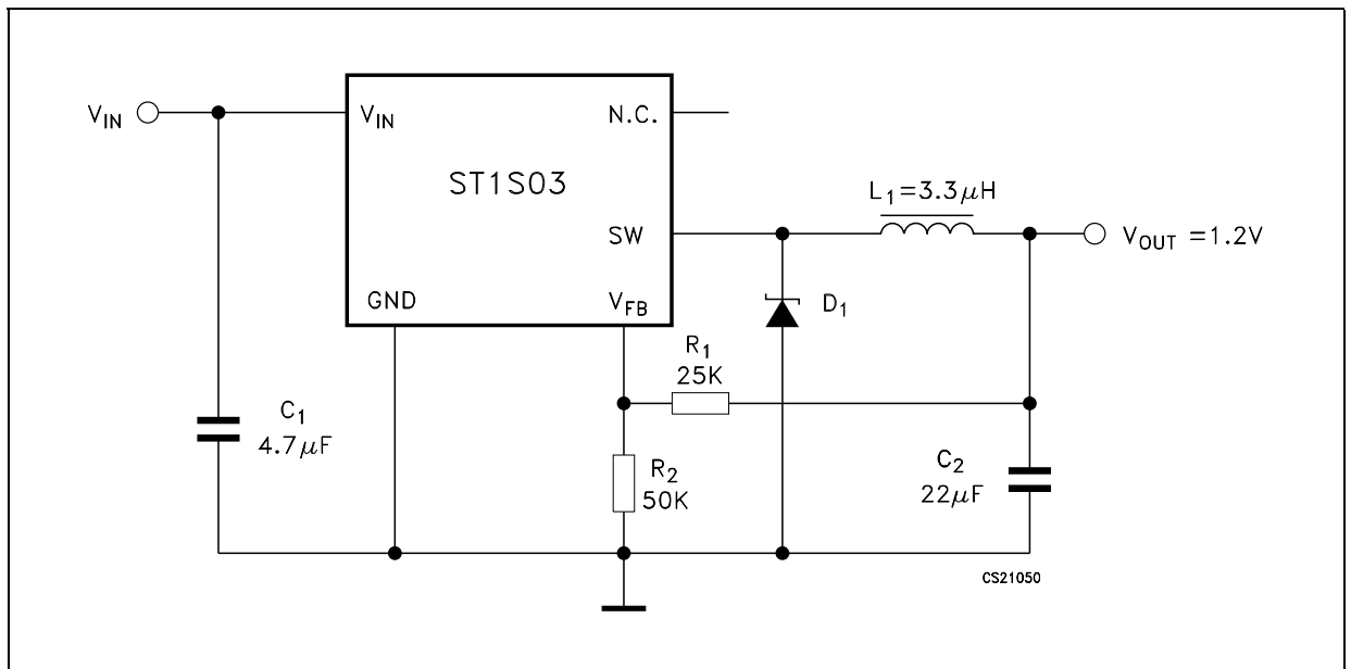
Figure 3: Application Circuit
