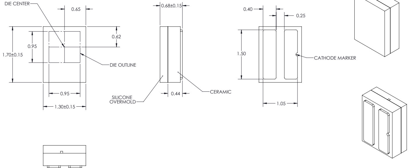
Figure 1. Package outline drawing.
