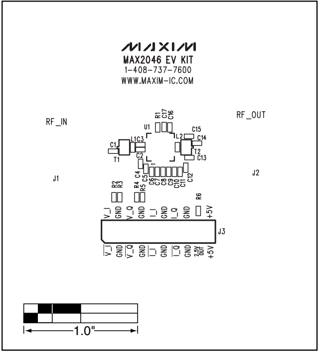
Figure 10. MAX2046 EV Kit Component Placement Guide—Top Silkscreen
