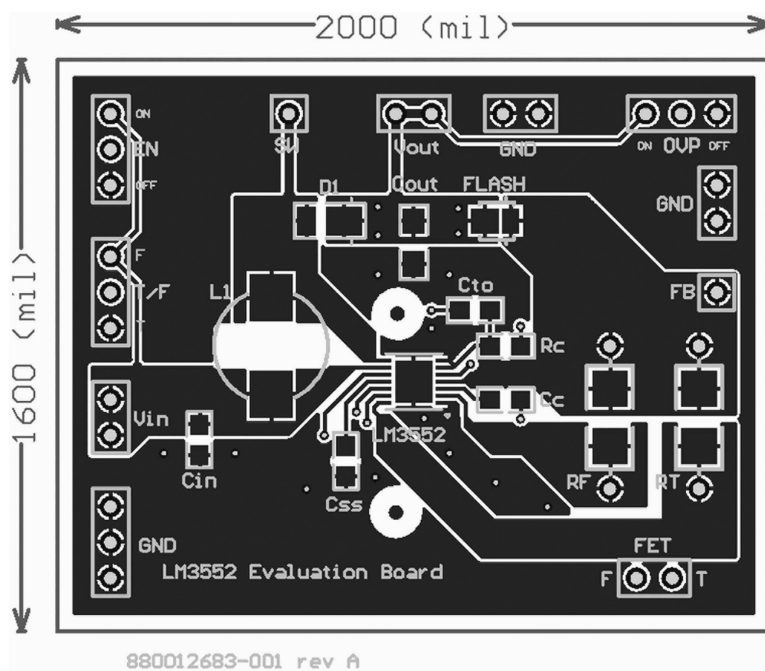
Figure 1. Top Layer
