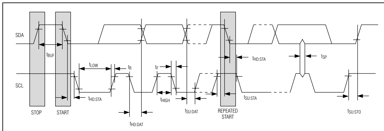
Figure 5. I²C AC Characteristics
