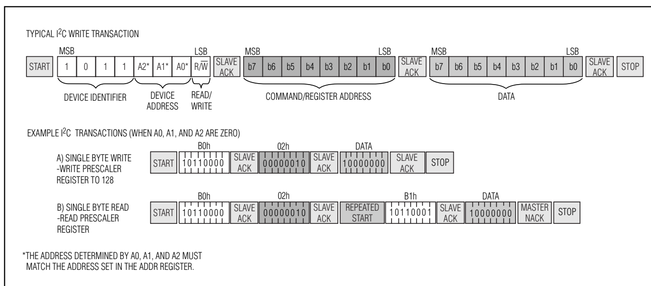
Figure 6. I²C Transactions
