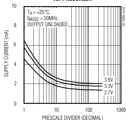
SUPPLY CURRENT vs. PRESCALER
