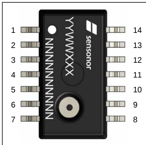
Figure 11.7 Pin configuration, top view
