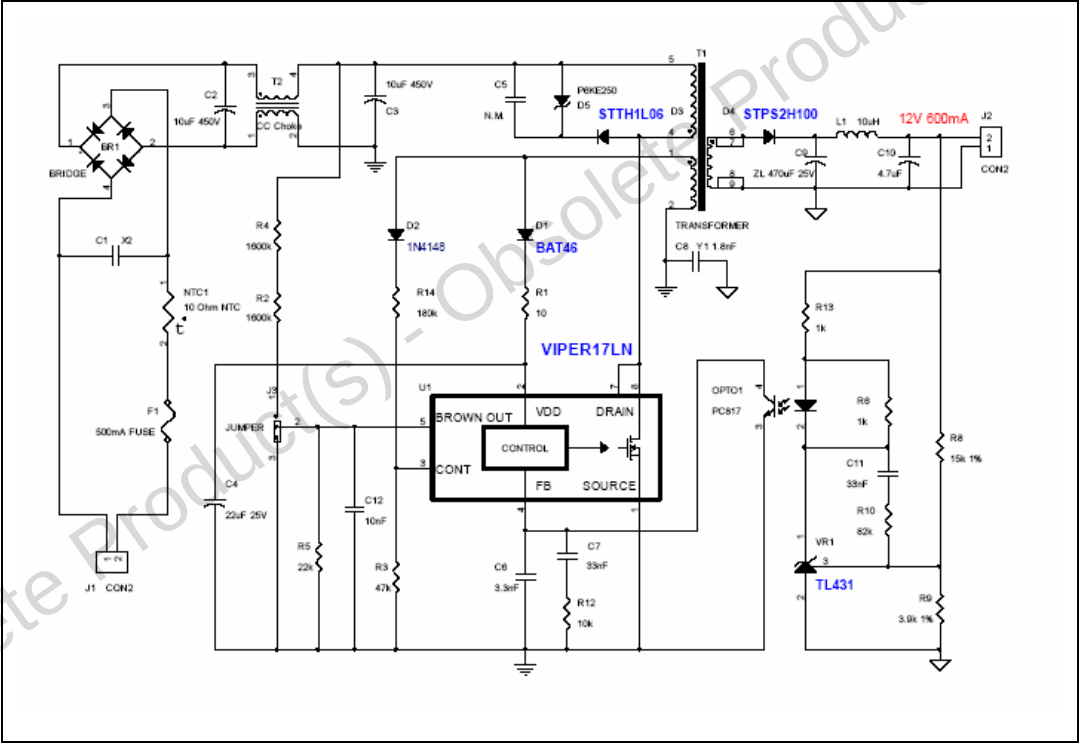
Figure 1. EVALVIPER17L-7W schematic
