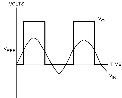
FIGURE 2. LMV7291 Basic Comparator
