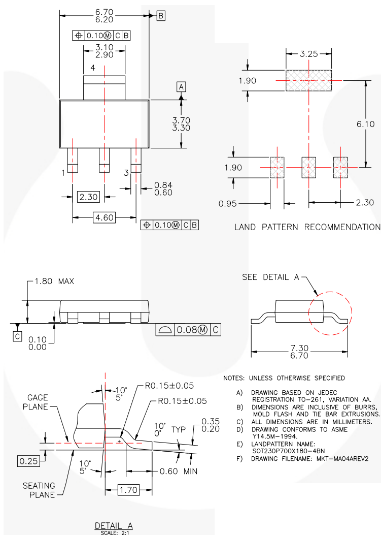
Figure 17. MOLDED PACKAGING, SOT-223, 4-LEAD (ACTIVE)
