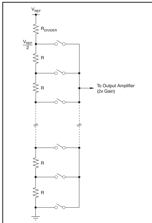
Figure 93. Resistor String
