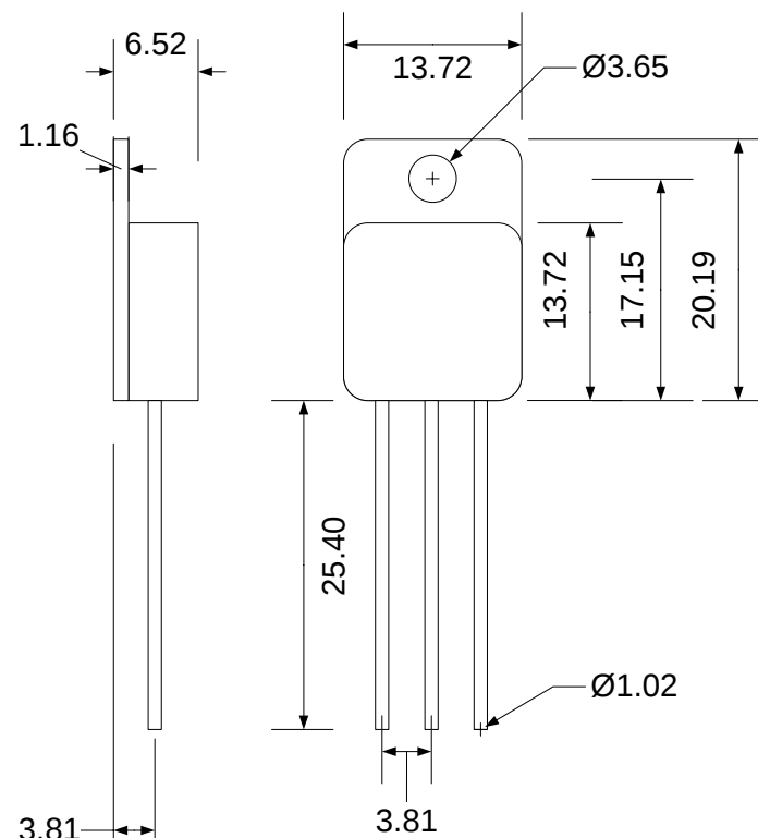
TO254 (mm +/- 10%)
