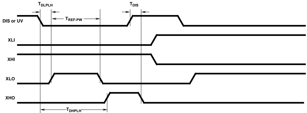
FIGURE 3. DISABLE FUNCTION
