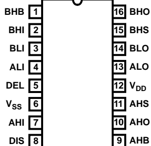
HIP4082 (PDIP, SOIC) TOP VIEW
