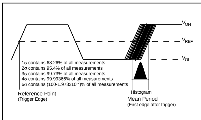
Period Jitter
