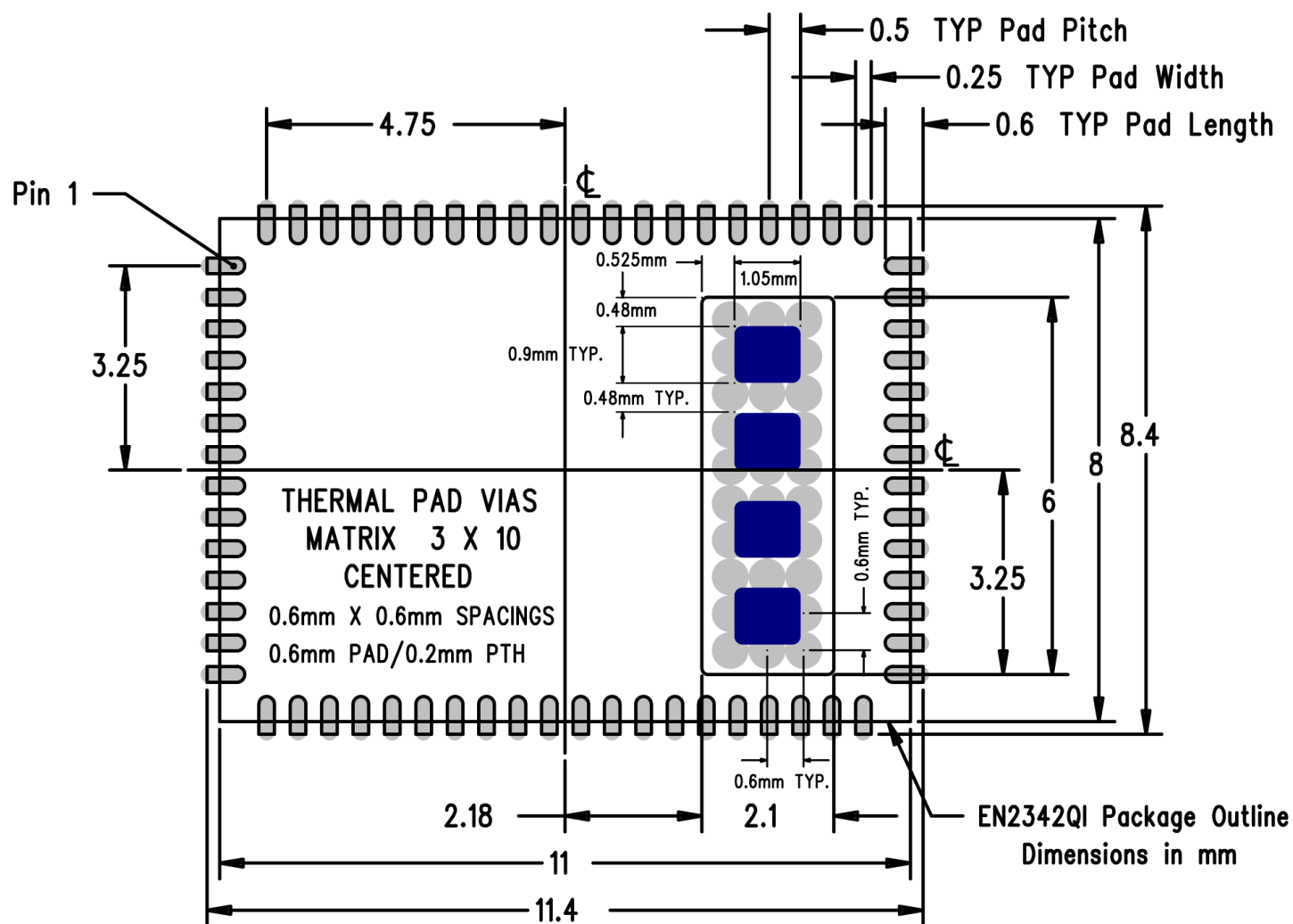
Figure 13: EN2342QI PCB Footprint (Top View)
