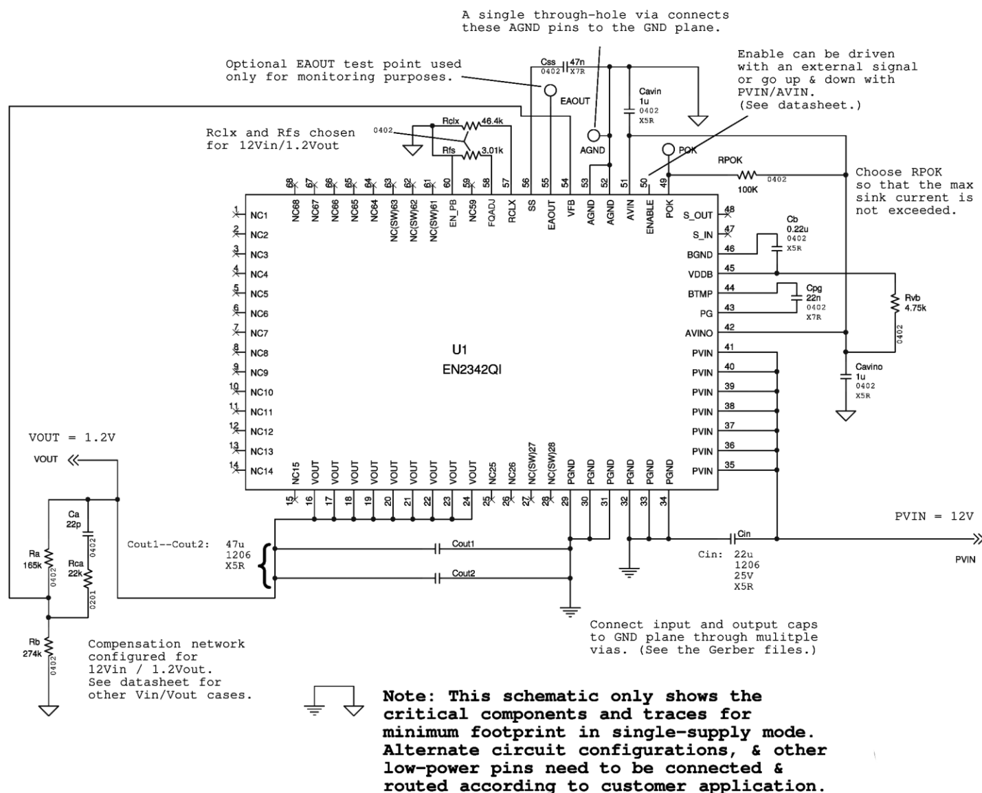
Figure 10: Engineering Schematic with Engineering Notes
