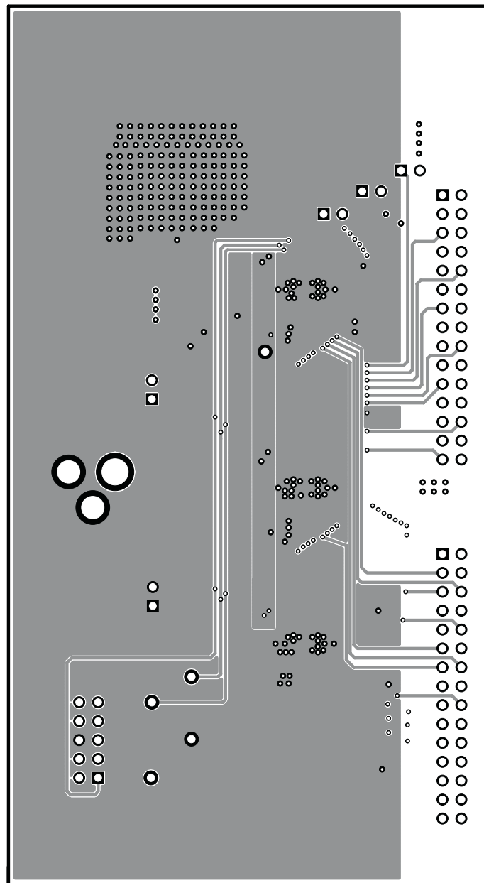
Figure 9. Layer 3 Routing
