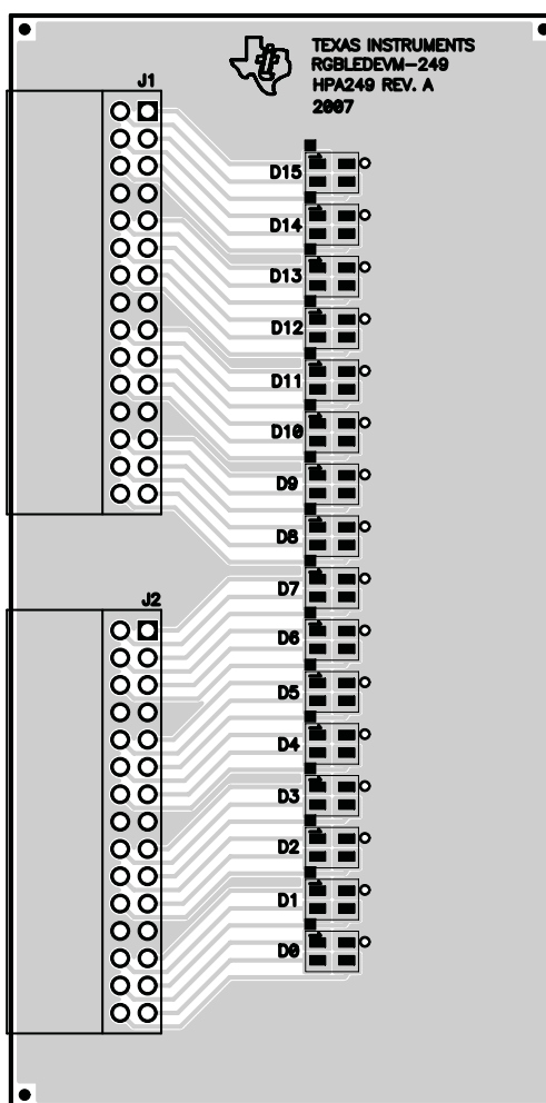
Figure 11. Assembly Layer Routing
