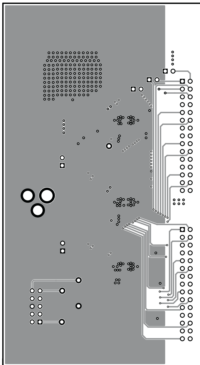
Figure 8. Layer 2 Routing
