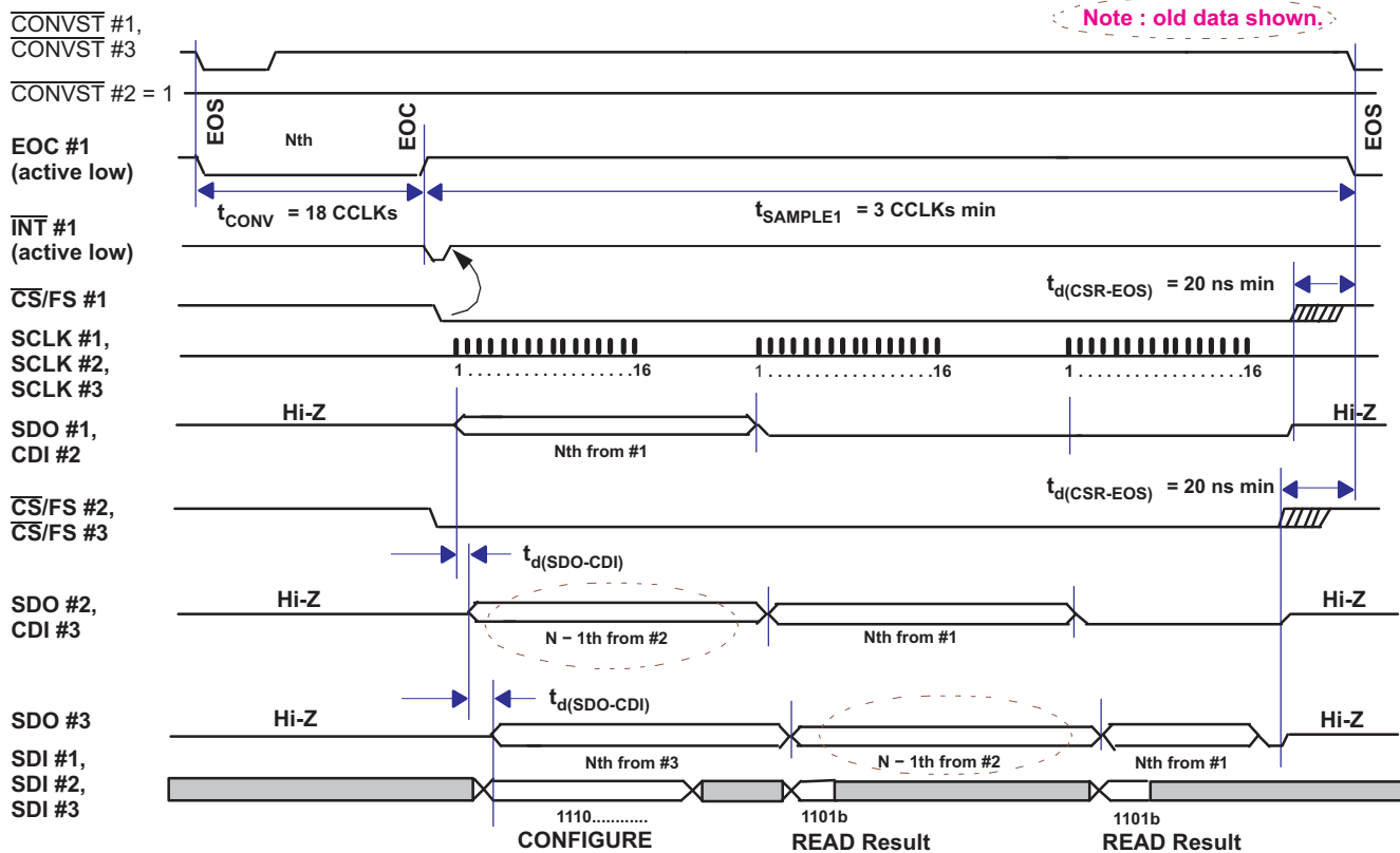
Figure 62. Simplified Cascade Timing (Separate \overline{\text{CONVST}} )
