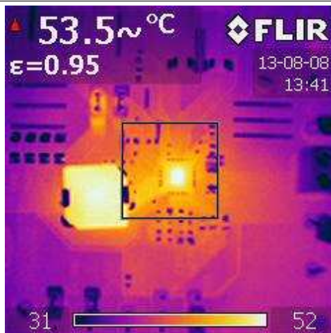
Figure 60. Thermal Signature of TPS65286EVM, T_A = \text{Room Temperature} , V_{IN} = 24\text{ V} , V_{OUT} to V_{SW\_in} = 5\text{ V}/0\text{ A} , I_{SW\_OUT1/2} = 1.2\text{ A} EVM Board: 4-Layer PCB, 1.6 mm Thickness, 2 oz. Copper Thickness, 65-mm x 65-mm Size, 25 Vias at Thermal Pad
