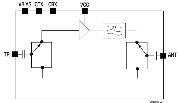
Figure 1. SKY66111-11 Functional Block Diagram
