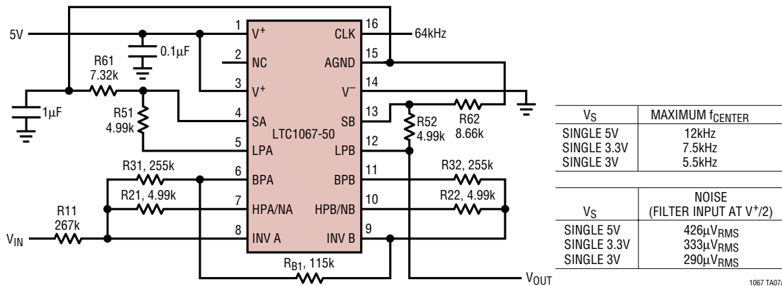
Single Supply, 4th Order Bandpass Filter
