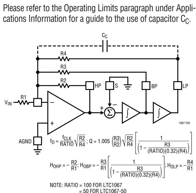
Figure 5. Mode 3, 2nd Order Section Providing Highpass, Bandpass and Lowpass Outputs
