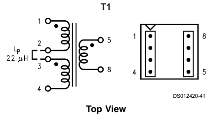
FIGURE 25. Renco RL-5530
