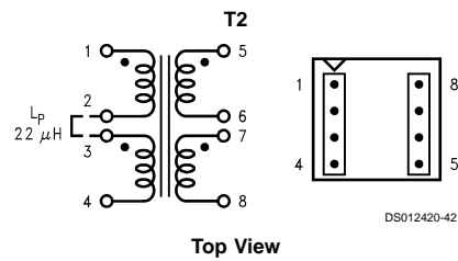
FIGURE 26. Renco RL-5531
