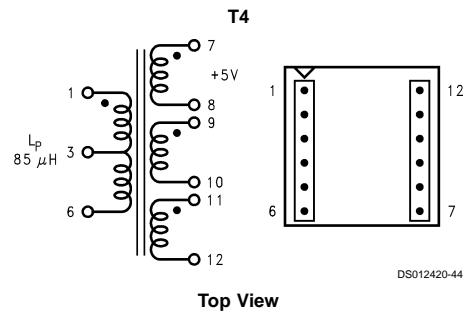
FIGURE 28. Renco RL-5535
