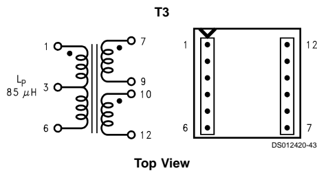
FIGURE 27. Renco RL-5534
