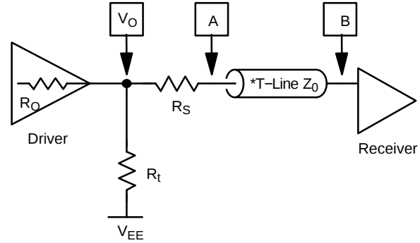
Figure 14. Series Termination
