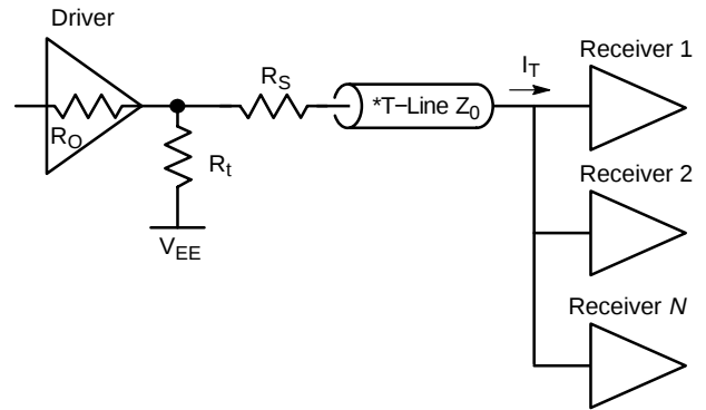
Figure 18. Noise Margin Loss Example
